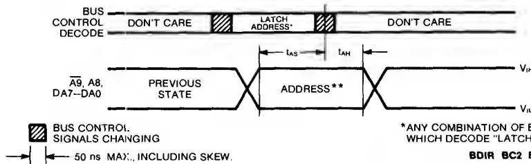
Fig. 9 LATCH ADDRESS TIMING
