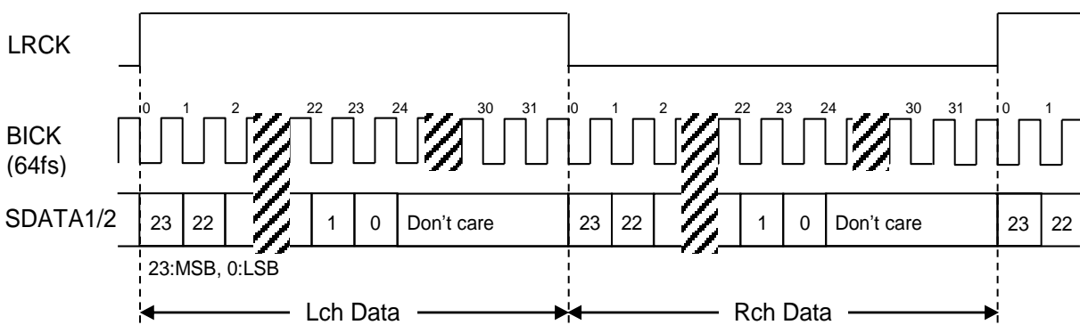
Figure 26. Mode 2 Timing
