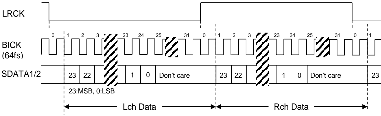
Figure 27. Mode 3 Timing
