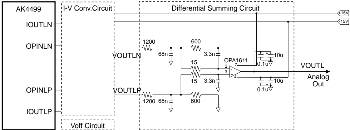
Figure 84. External 2nd Order LPF Circuit Example for PCM mode ( f_c = 112 \text{ kHz (typ)} , Q = 0.692 \text{ (typ)} )
