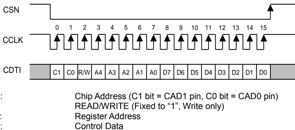
Figure 71. Control I/F Timing
