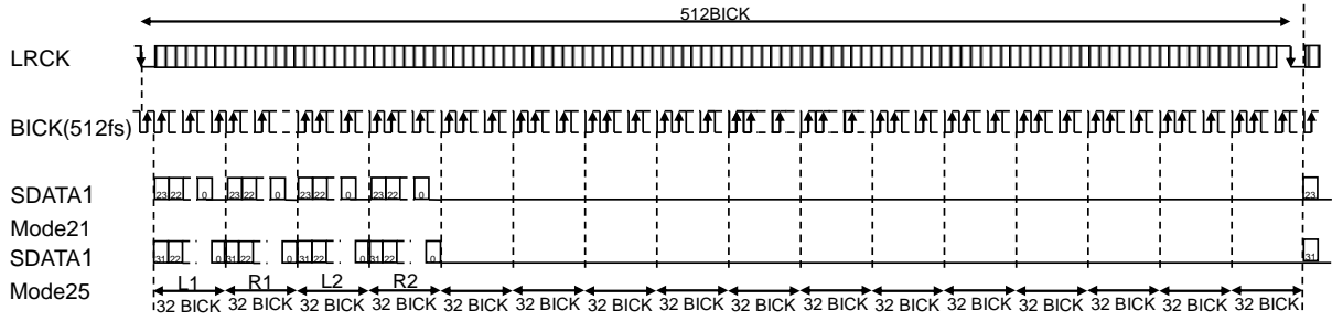
Figure 38. Mode 21/25 Timing
