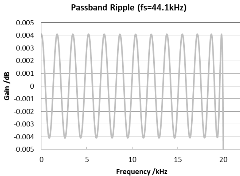
Figure 3. Sharp Roll-Off Filter Pass Band Ripple
