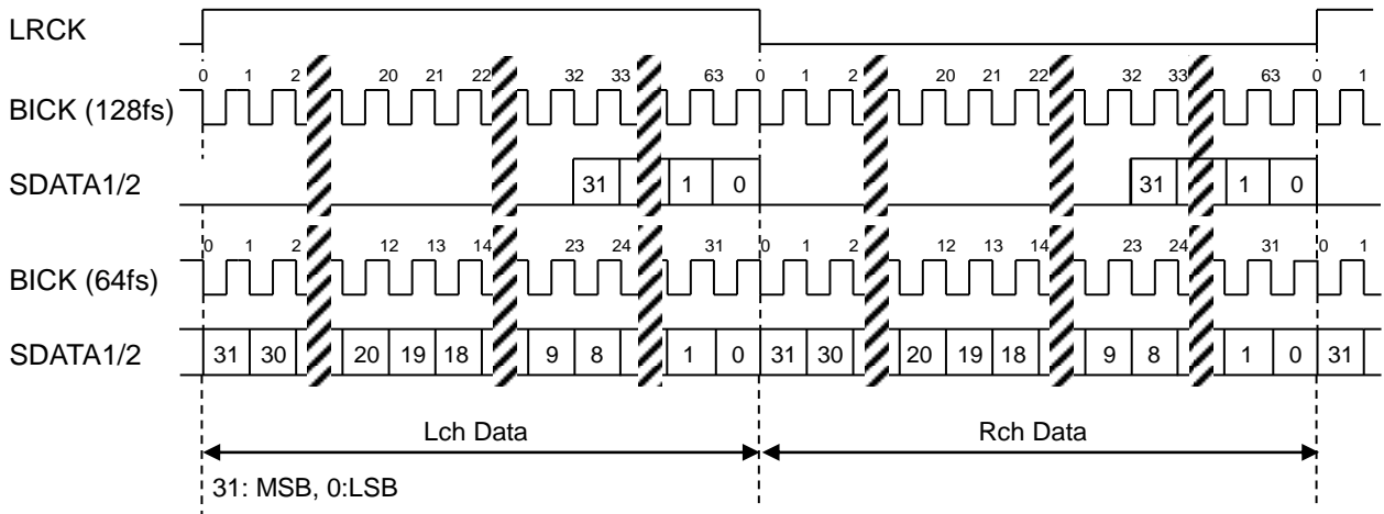
Figure 28. Mode 5 Timing
