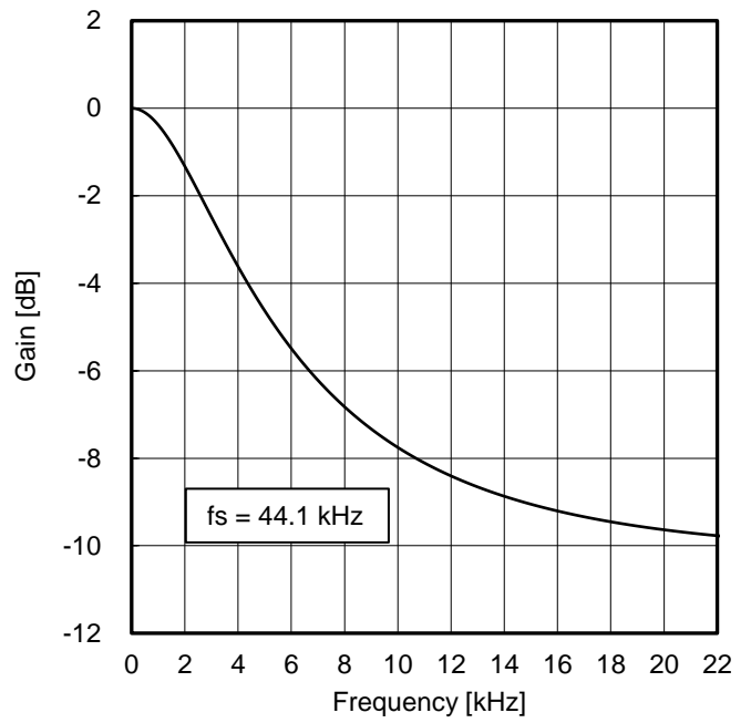
Figure 31. Gain vs Frequency
