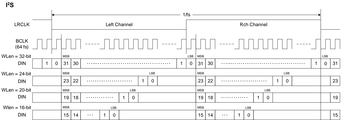
Figure 20. Audio Data Input Format: I²S
