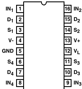
DG411, DG412, DG413 (PDIP, SOIC, TSSOP) TOP VIEW
